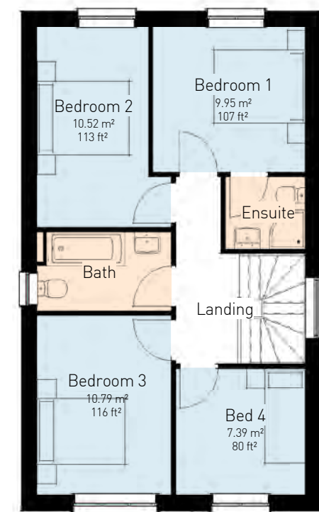
First Floor 1 : 100
