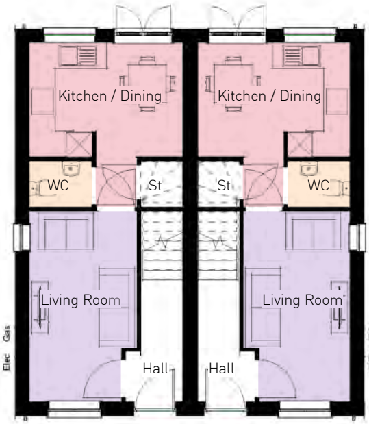
Ground Floor 1 : 100
