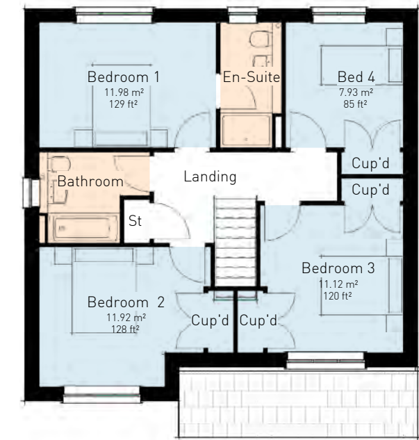
First Floor 1 : 100
