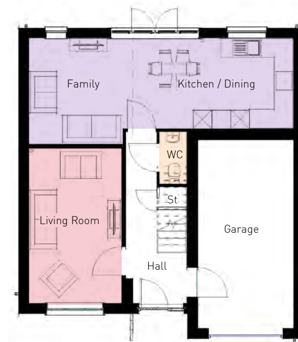
Ground Floor 1 : 100
