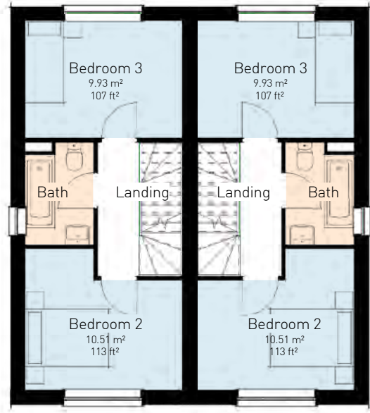
First Floor 1 : 100
