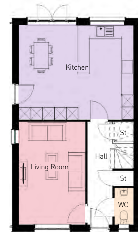
Ground Floor 1 : 100
